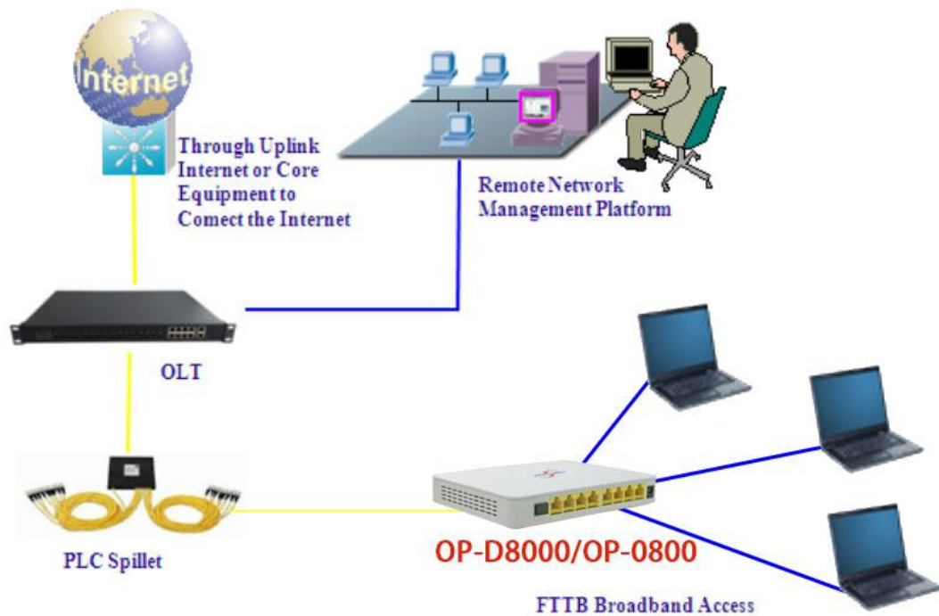
Figure: OP-D4000D/ OP-D8000&OP-D0800 Application Diagram
